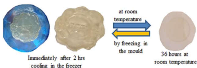
Figure 9. A reversible reaction.
