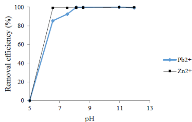
Figure 4. Effect of pH on the efficiency of removing \text{Pb}^{2+} and \text{Zn}^{2+} with initial concentrations of 500 mg/L from their two-component aqueous solutions
